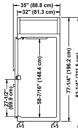
Section View - All Models
